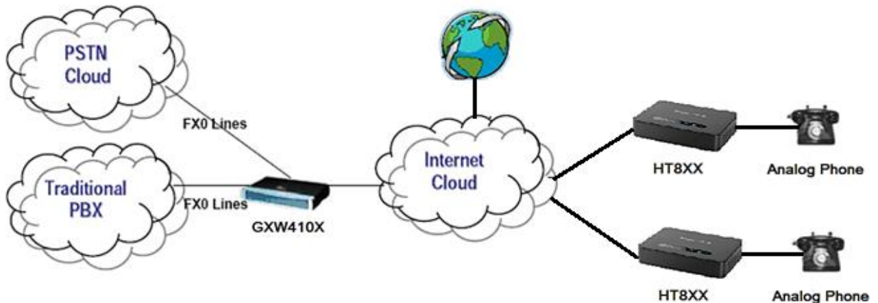
Figure 16: Peering Multiple HT8XX with GXW410X
