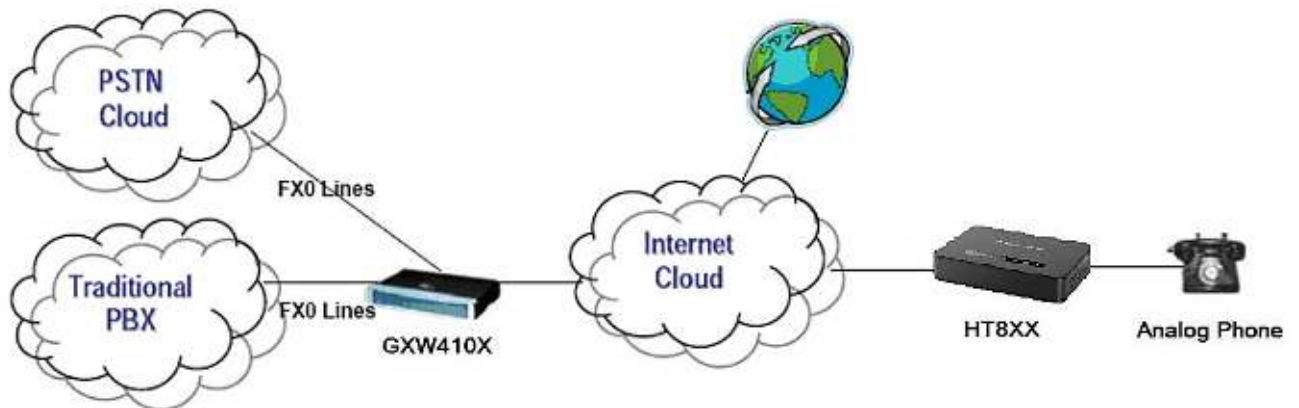
Figure 3 : Peering one HT8XX with GXW410X
