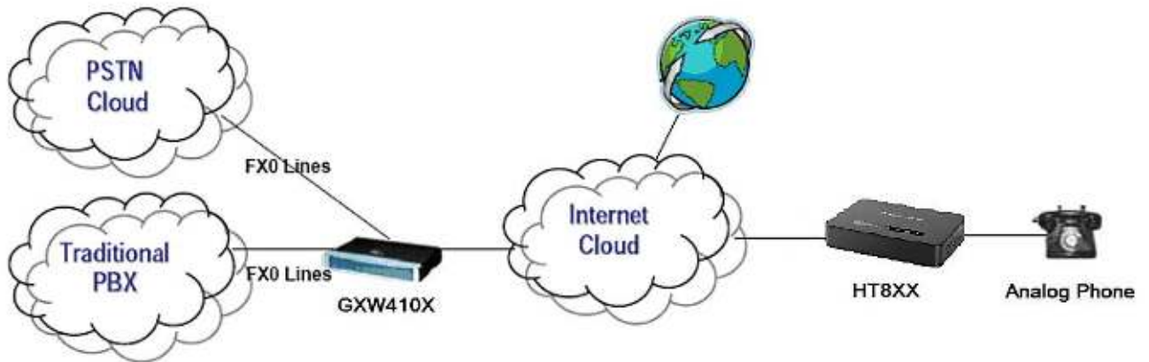
Figure 1 : Scenario 1: Peering one HT8XX with GXW410X
