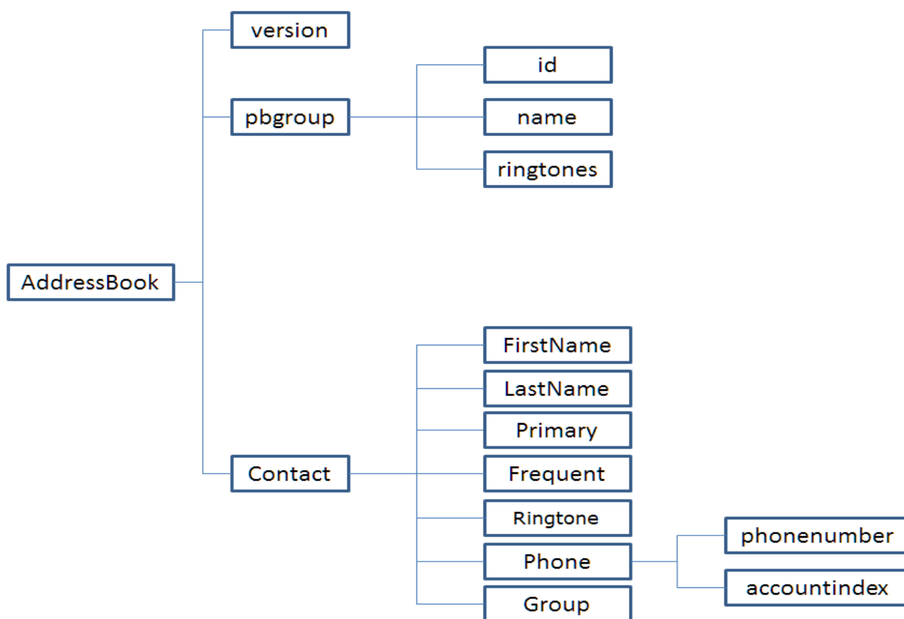
Figure 4: Main XML Hierarchy
