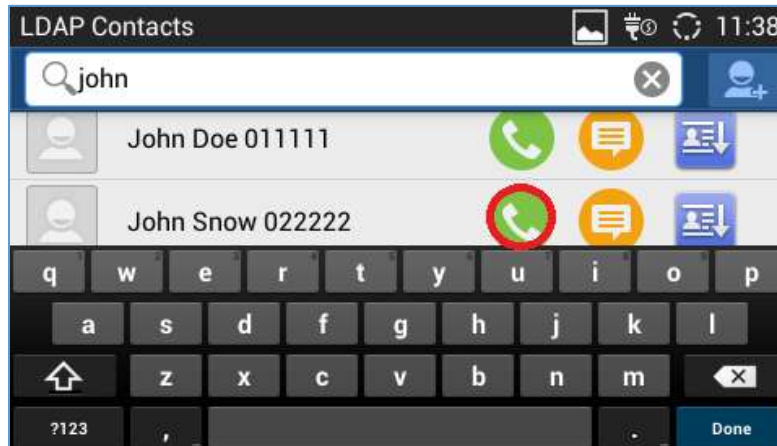
Figure 21: LDAP Calls
