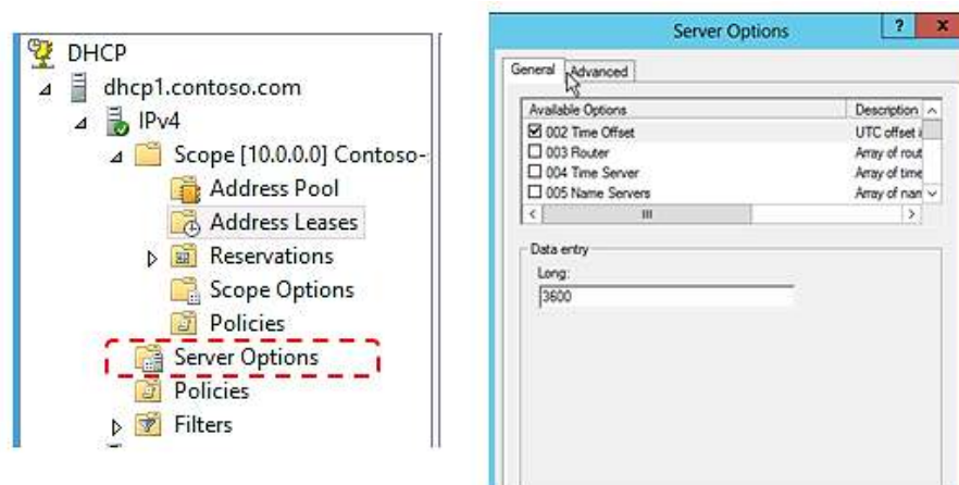
Figure 7 : Server Options
