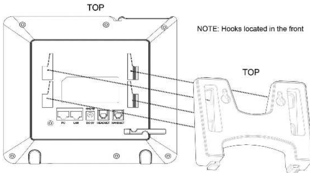
Figure 3: GXP16xx Wall Mount installation
