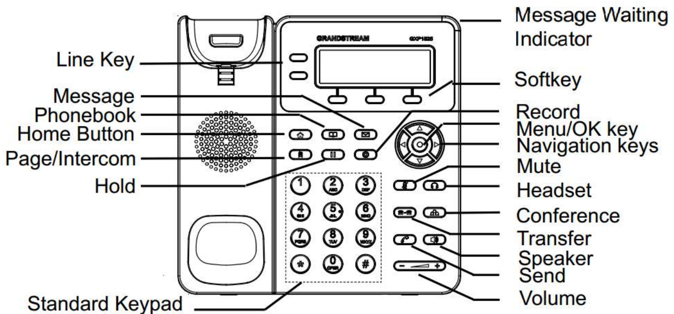
Figure 5: GXP16xx Front View (GXP162x as example)
