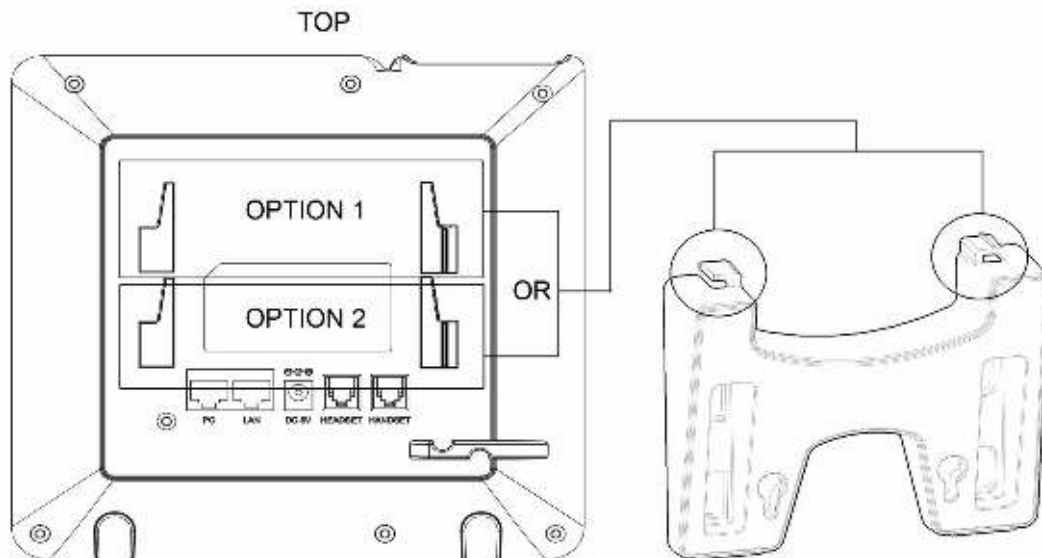
Figure 2: GXP16xx Stand Installation
