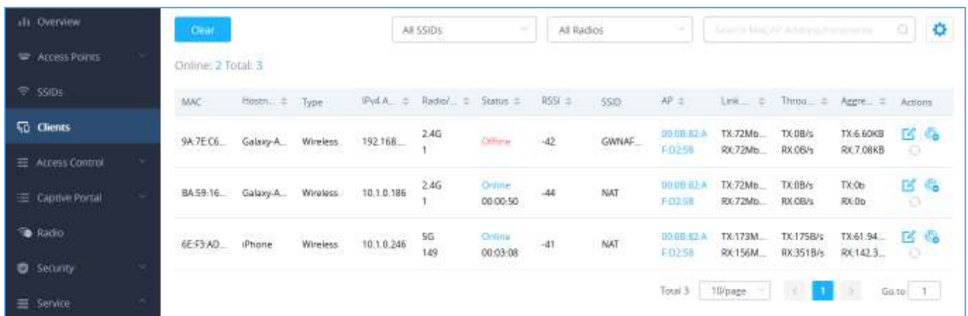
Figure 7: NAT Pool-Client
