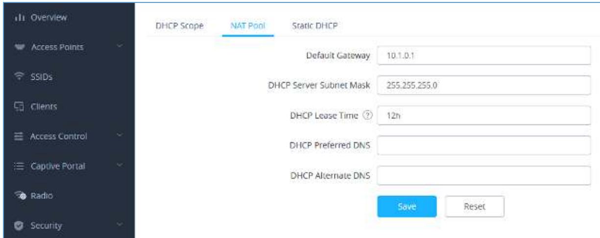
Figure 6: NAT Pool
