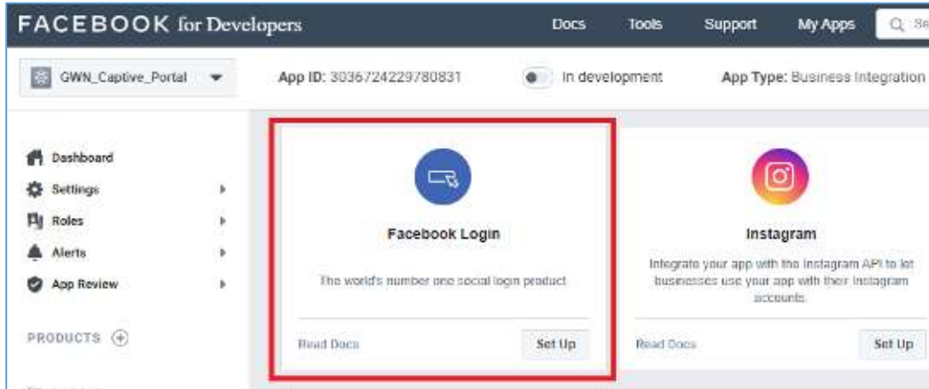
Figure 9: Add "Facebook login" product to your App
