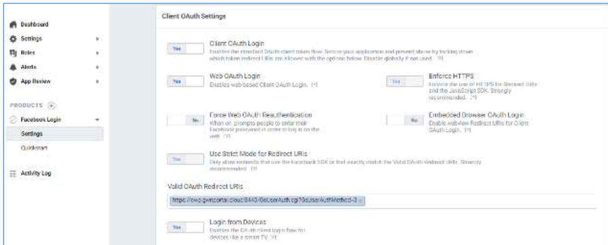
Figure 11: Facebook Login Settings - Valid OAuth redirect URIs
