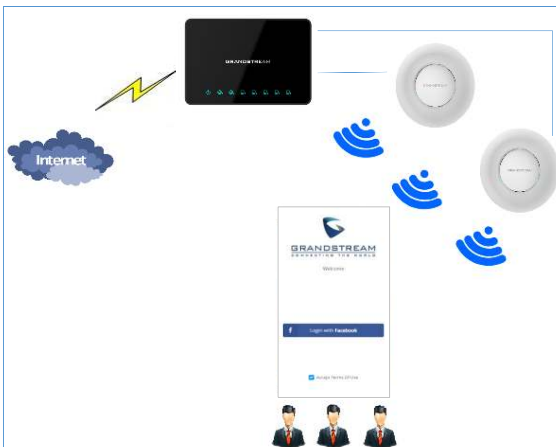
Figure 1: General Architecture
