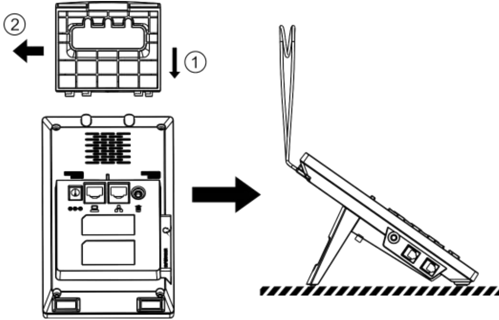
Figure 1 - Bracket installation
