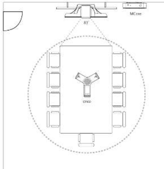
For Medium-to-large conference room (8-18 people)
