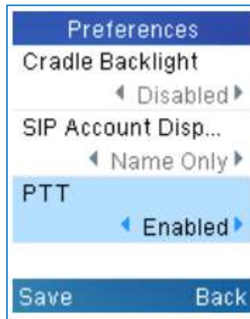
Figure 42: Enable PTT
