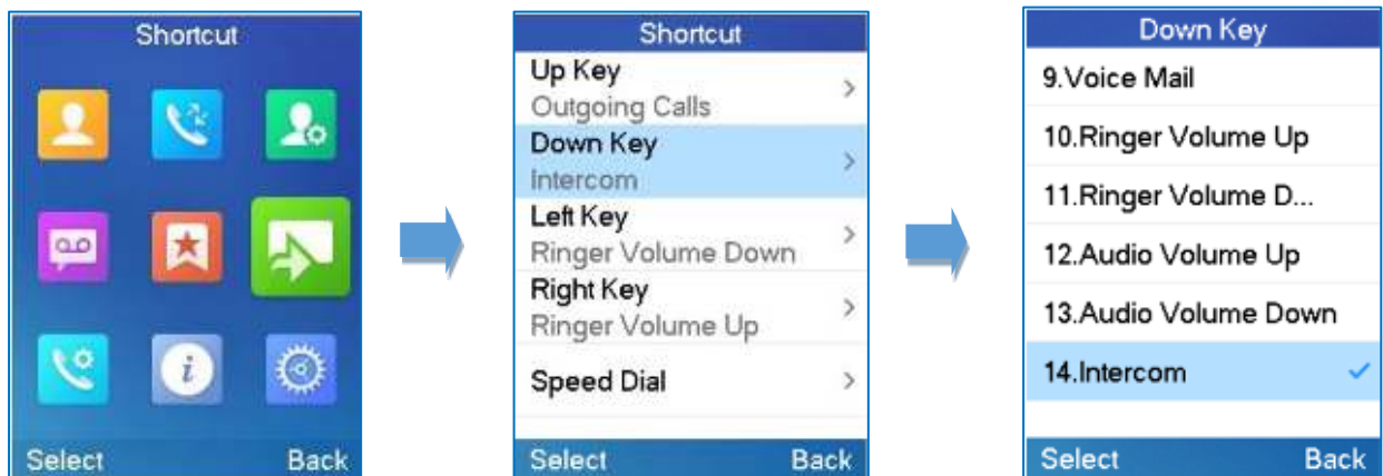
Figure 39: Shortcut Setting
