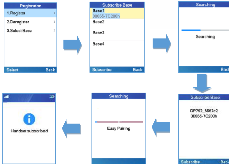
Figure 11: Registration Process
