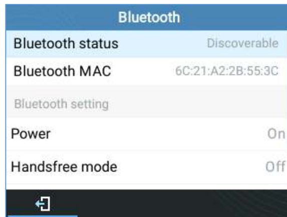
Figure 79: Bluetooth Status
