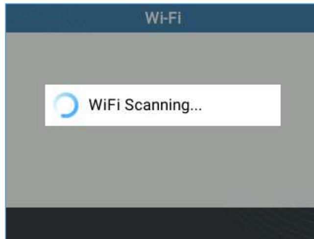
Figure 83: Wi-Fi Scanning
