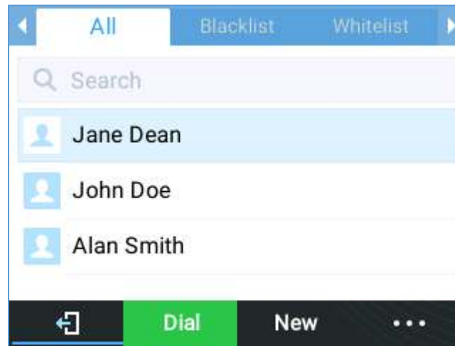
Figure 67: Before Search
