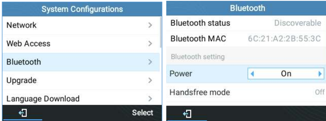
Figure 75: Bluetooth feature
