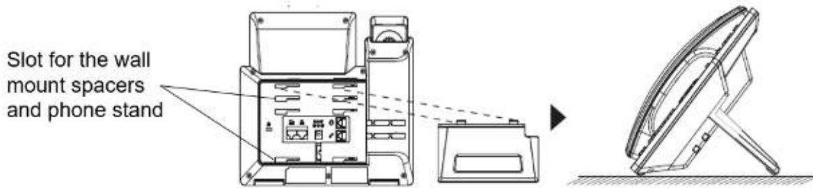
Figure 2: phone Stand and Mounting Slots on the GRP261X
