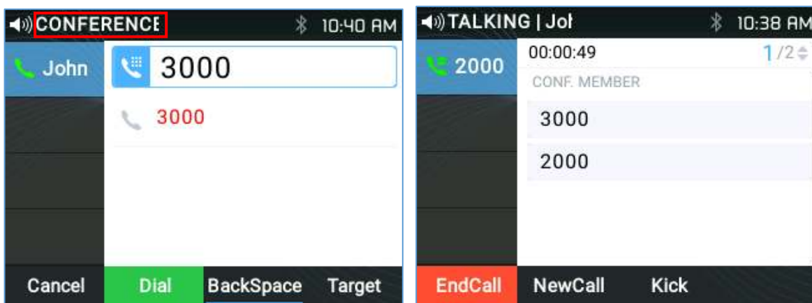
Figure 30: Established Conference
