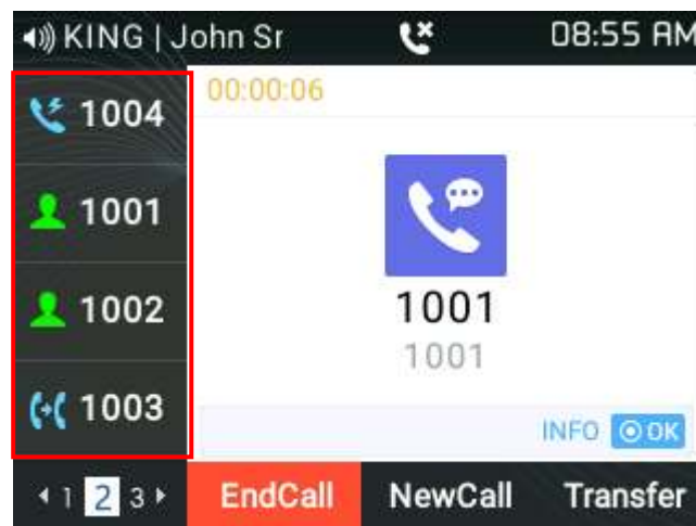
Figure 56: VPK Paging
