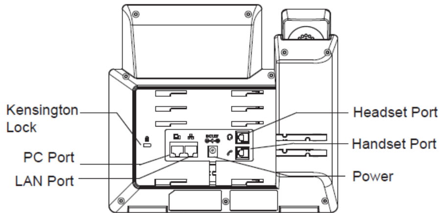
Figure 4: GRP261X Back / Side View
