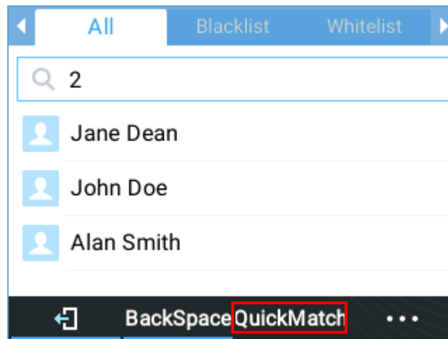
Figure 68: QuickMatch
