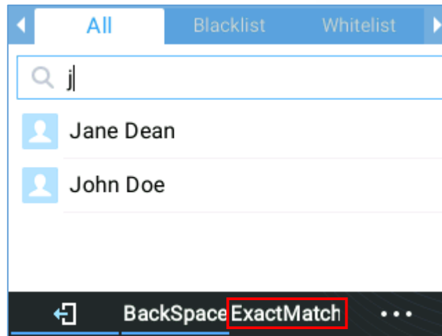
Figure 69: ExactMatch
