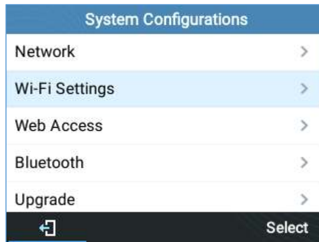
Figure 81: Wi-Fi feature
