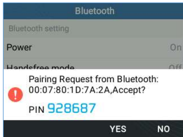
Figure 79: Bluetooth Status
