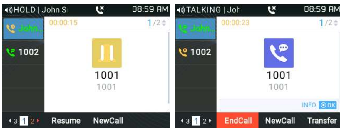
Figure 58: Line Switching
