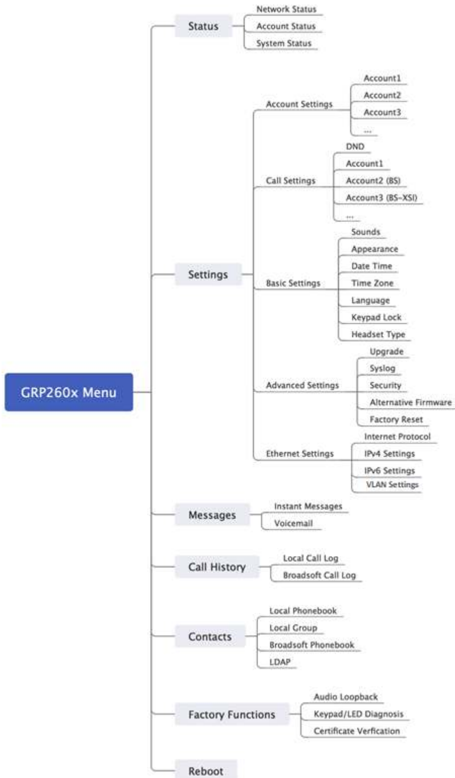
Figure 10: Keypad Menu Configuration Flow
