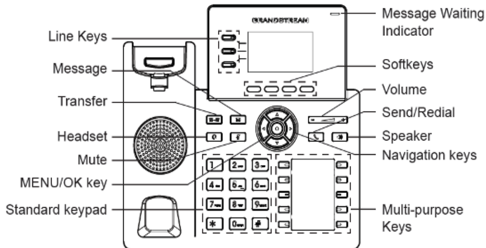
Figure 9: GRP2604 Keyboard
