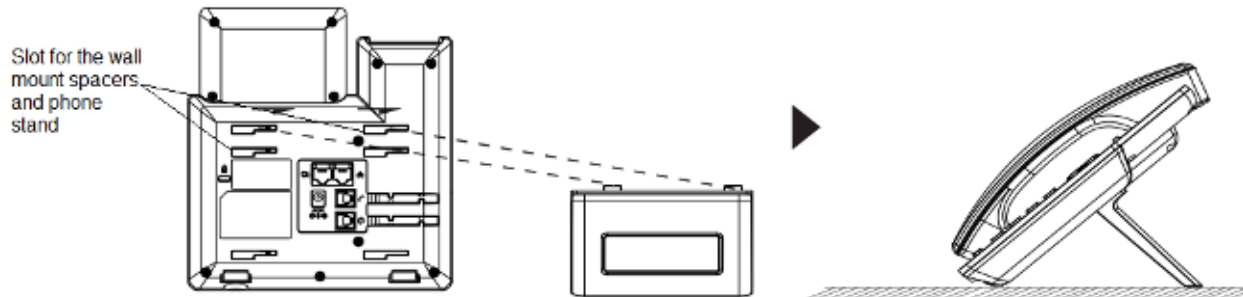
Figure 2: phone Stand and Mounting Slots on the GRP260x
