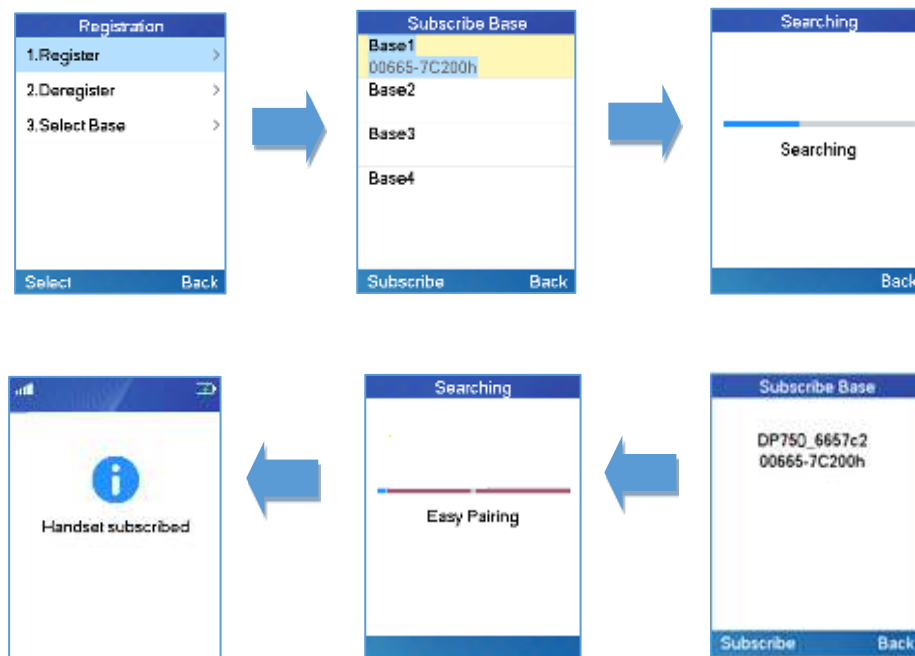
Figure 10: Registration process
